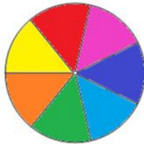
Disque de Newton immobile Figure 1
